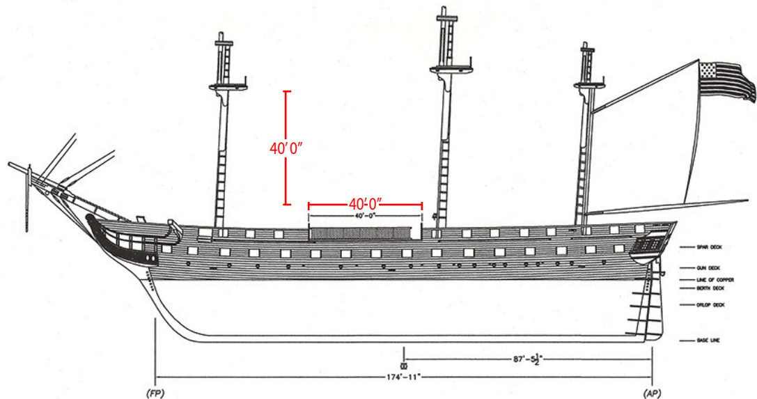
ELEVATION "12-A" U.S. FRIGATE CONSTITUTION
